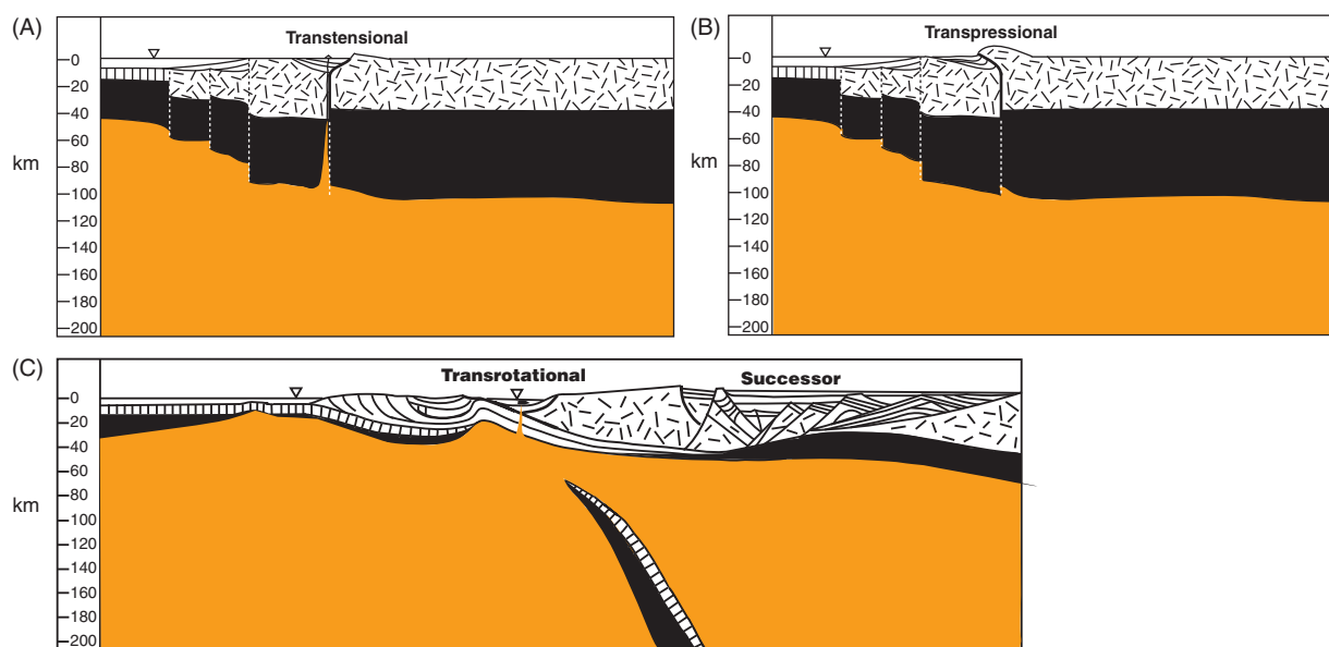
Fig. 1.5. True-scale actualistic analog models for sedimentary basins in transform and miscellaneous settings. These cross sections are based on the Miocene to Holocene evolution of southern California (Ingersoll, 2008b); many other tectonic settings are common for transtensional and transpressional basins. Transrotational basins are less common; the three-plate interactions depicted in (C) are unique on Earth today. Successor basins may form following cessation of any tectonic activity; shown in (C) is the southern Basin and Range of the USA, where undeformed Neogene to Holocene strata overlie tilted fault blocks and strata of the older extensional regime. Symbols same as in Figure 1.3.
